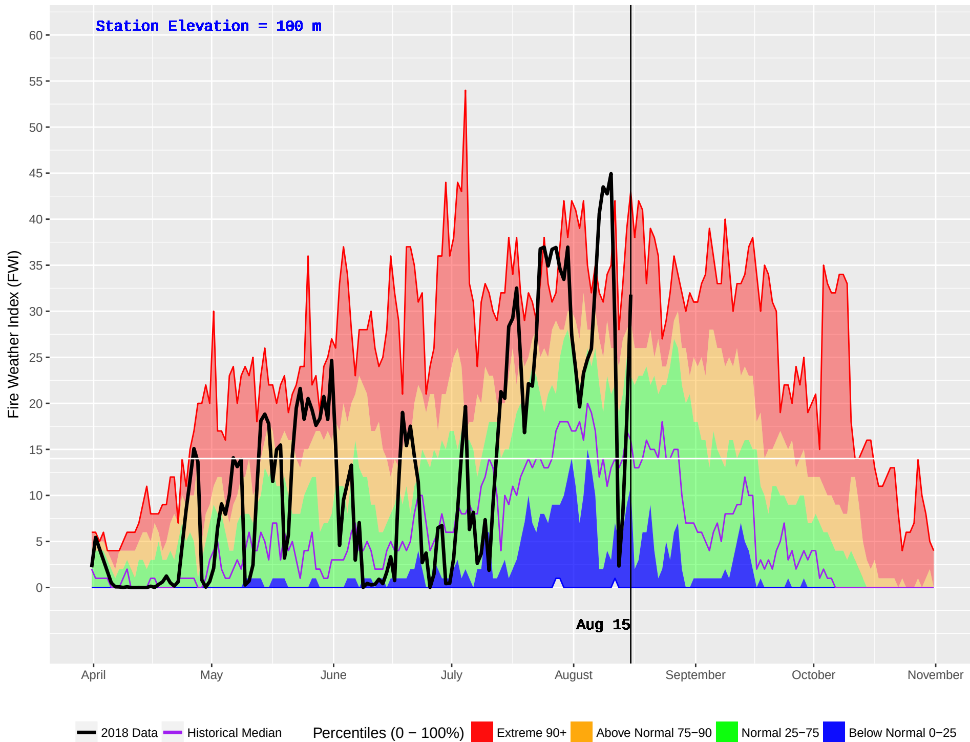
BEAVER CREEK (37) : Historical (1987–2016) and Current (2018) Daily Fire Weather Index (FWI)
