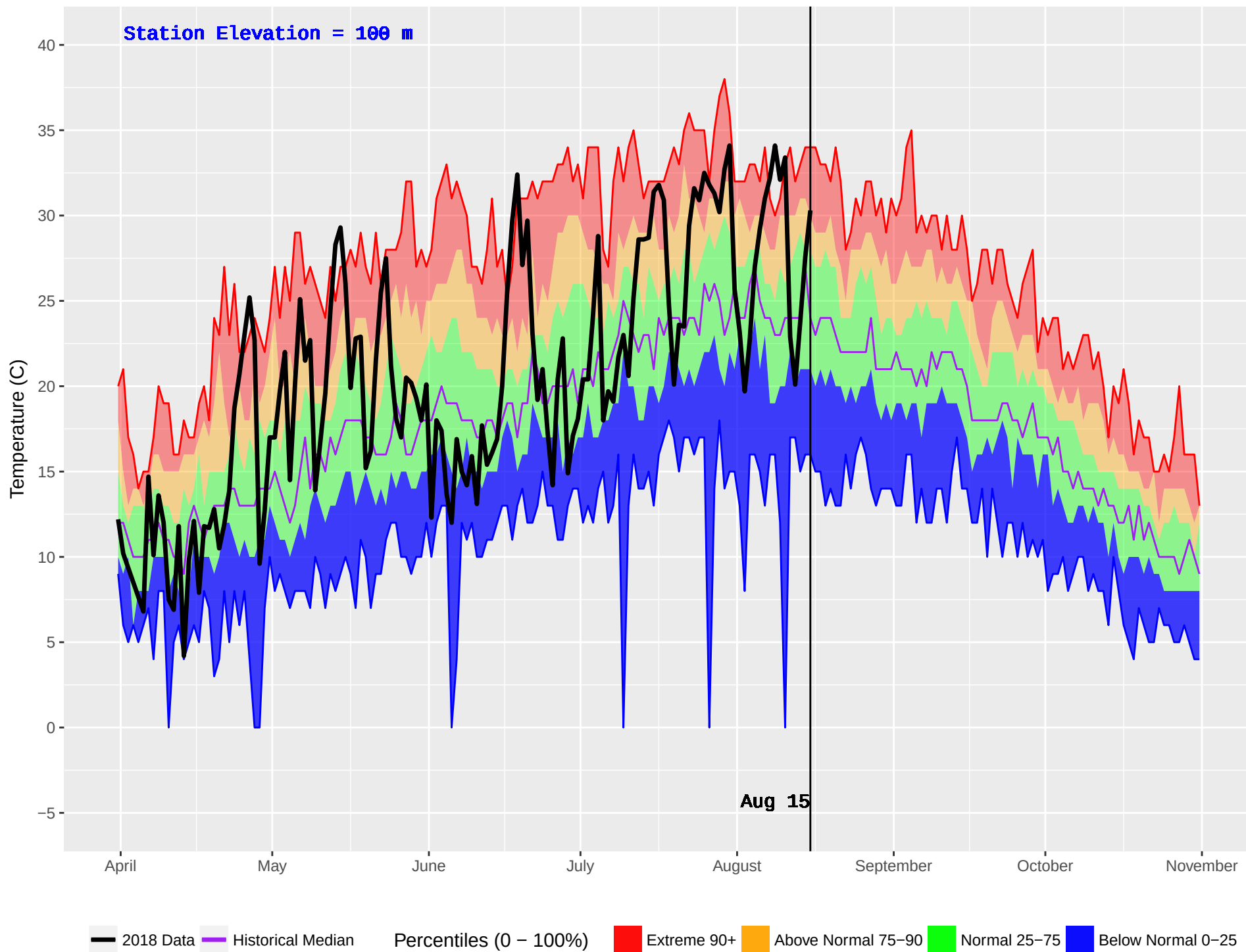
BEAVER CREEK (37) : Historical (1987–2016) and Current (2018) Daily Temperature
